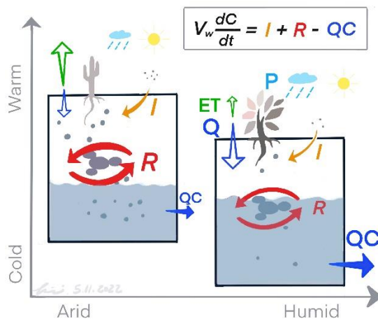
Figure 1: A conceptual model of a watershed hydro-biogeochemical reactor. Water originates from precipitation and travels via subsurface flow paths before re-emerging in rivers. Along its flow paths, water mobilizes solutes by interacting with roots, microbes, soil, and rocks. The dynamics of solute concentrations in the stored water ( V_w ) are therefore regulated primarily by two competing processes:
