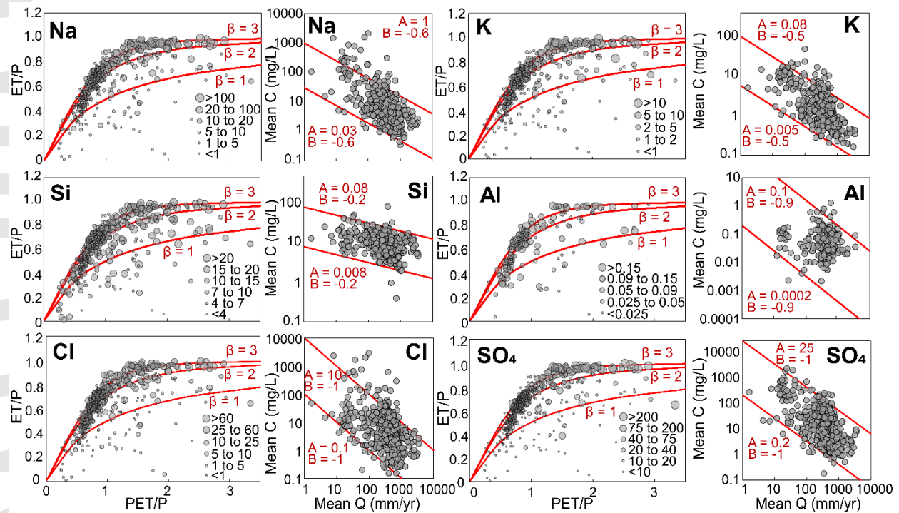
Figure 4. Geogenic solutes from weathering without thermodynamic limitation. Each solute has one pair of figures. The left figure of each pair is C_m within the Budyko framework. Red lines are from Equation (0) with different non-linearity indicator \beta . The positions of circles are determined by evaporative index (ET/P)
